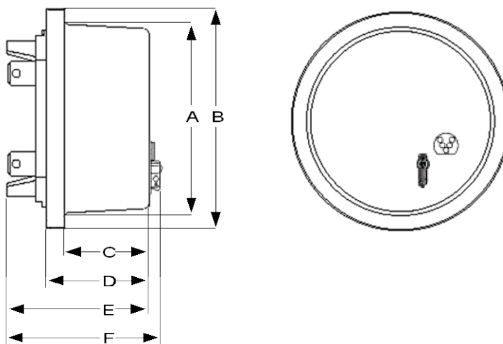
Figure 4: CP1SO (CP2SO) Dimensions
